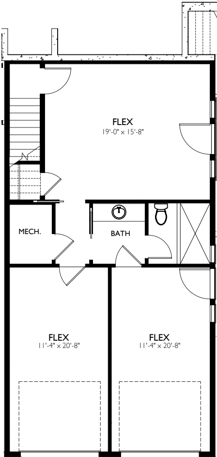
1ST FLOOR 8'-0" CLGs
