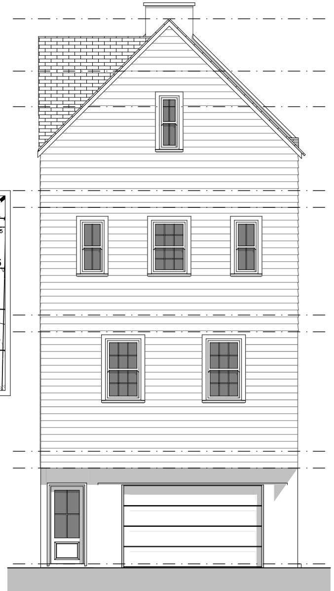
REAR ELEVATION \frac{1}{8}'' = 1'-0''
