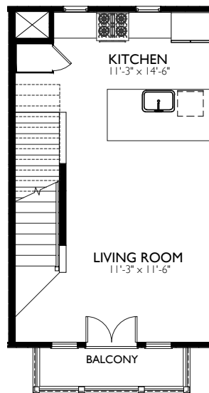
2ND FLOOR 10'-0" CLGs
