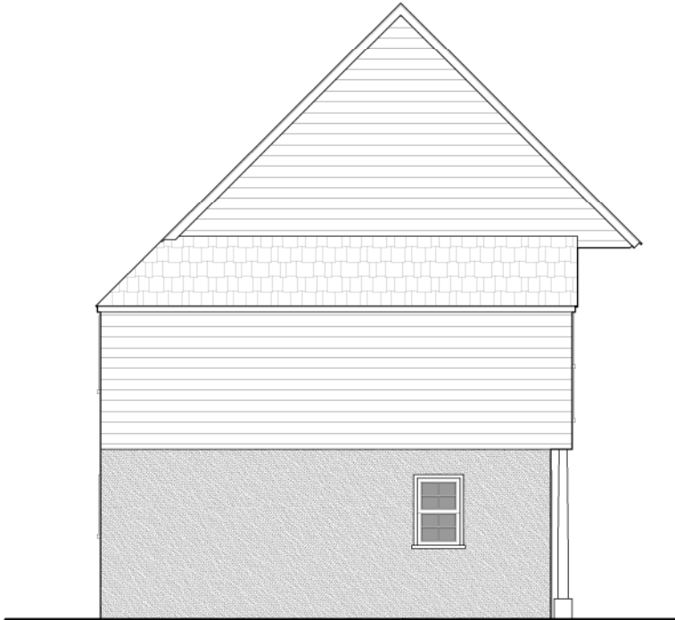
GARAGE LEFT ELEVATION
