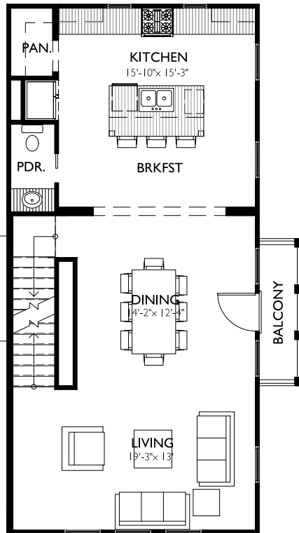
2ND FLOOR 10'-0" CLGs
