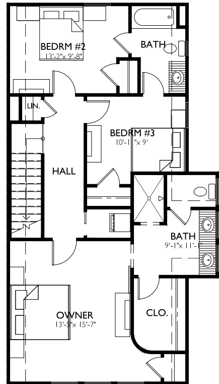
3RD FLOOR 9'-0" CLGs
