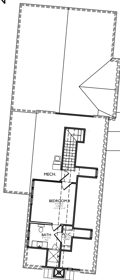
3rd FLOOR 8'-0" CLG
