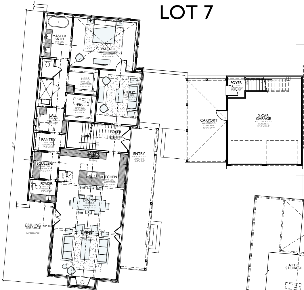
1ST FLOOR 11'-0" CLGs
