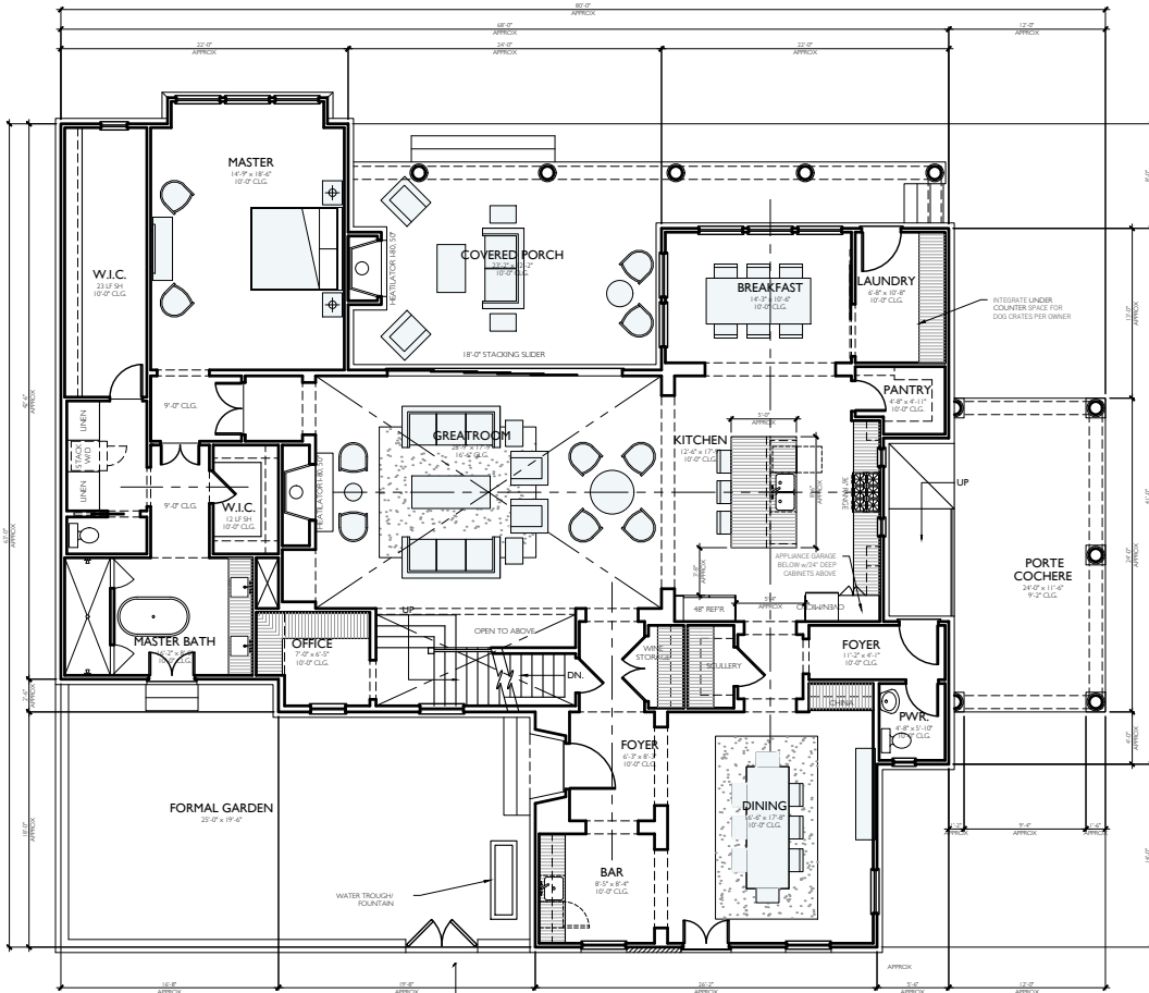
HOUSE - 1st FLOOR 10'-0" Ceilings
