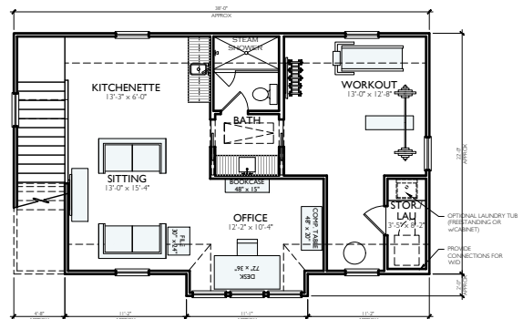
2nd FLOOR 9'-0" Ceilings
