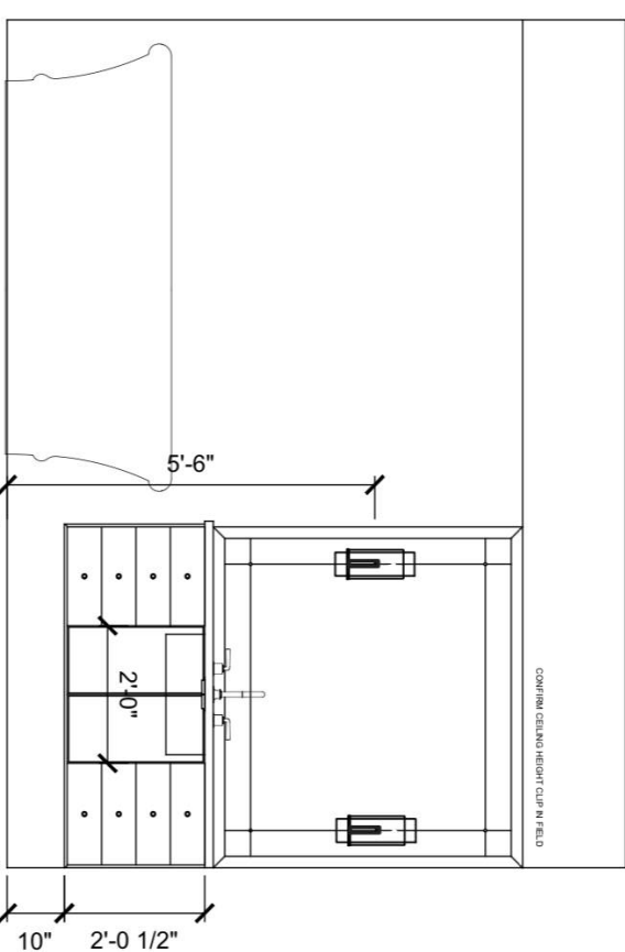
MASTER BATHROOM - HER SIDE
