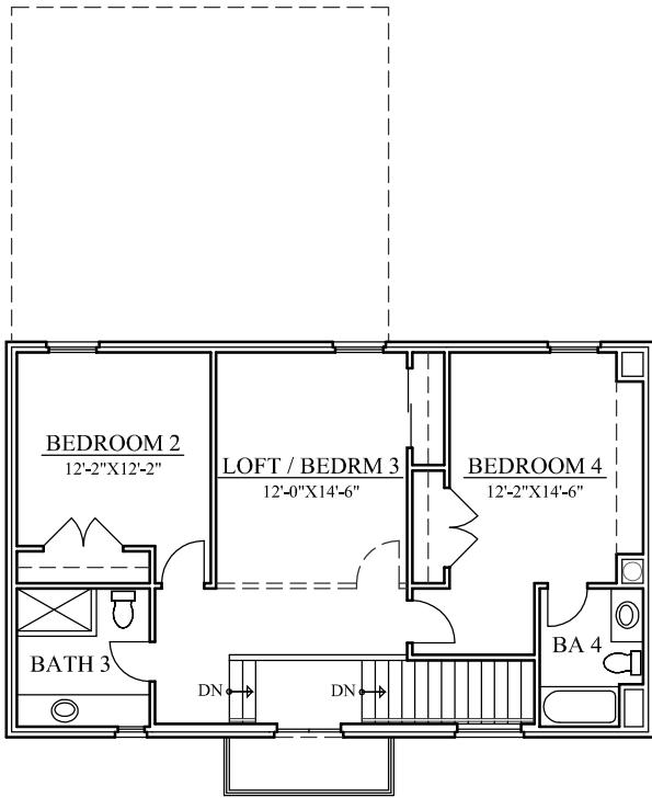
UPPER FLOOR PLAN 9'-0" CEILING
