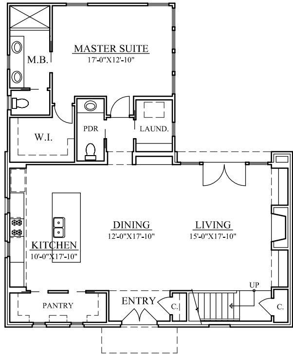
MAIN FLOOR PLAN 10'-0" CEILING
