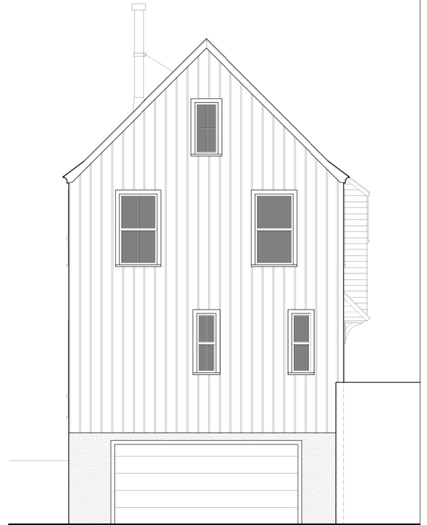
REAR ELEVATION
