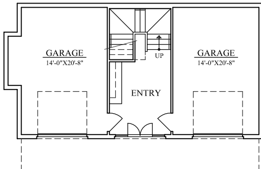
TERRACE FLOOR PLAN 8'-0" CEILING
