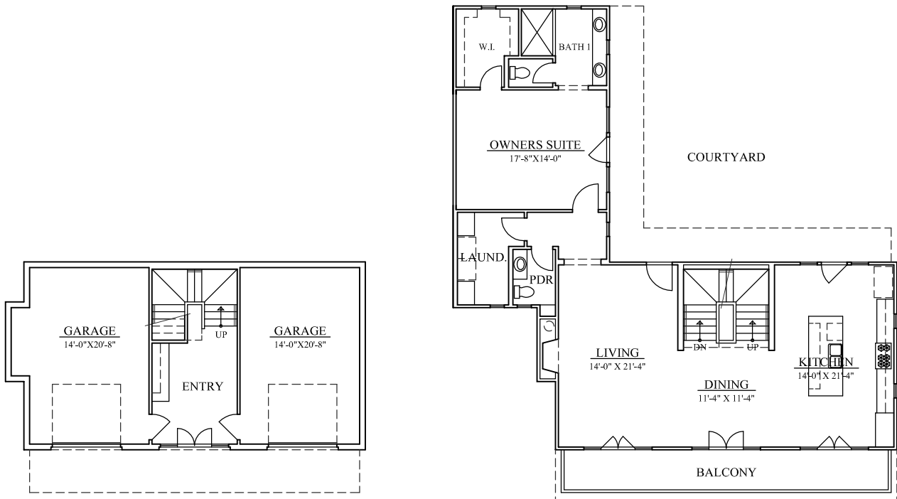
MAIN FLOOR PLAN 10'-0" CEILING
