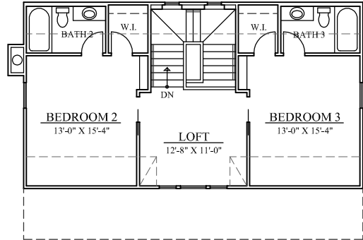
UPPER FLOOR PLAN 9'-0" CEILING
