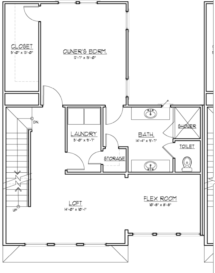
UPPER LEVEL FLOOR 9'-0" CEILING
