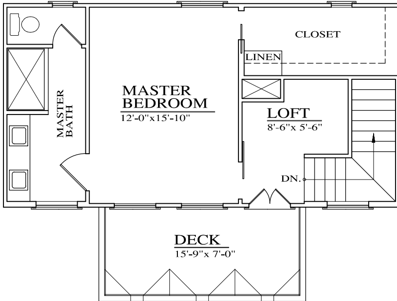
UPPER LEVEL 3RD FLOOR PLAN
