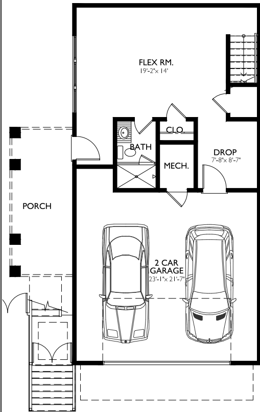
1ST FLOOR 8'-0" CLGs
